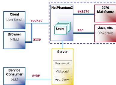
NetPhantomX® architecture
